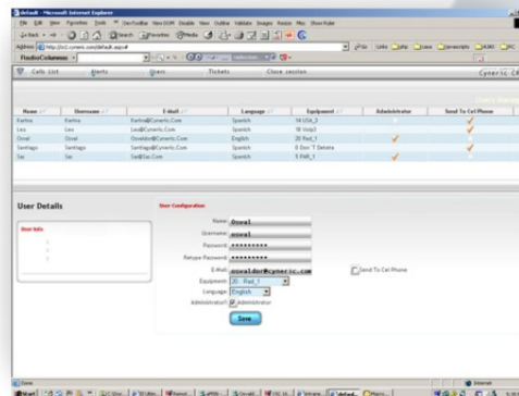
User details
