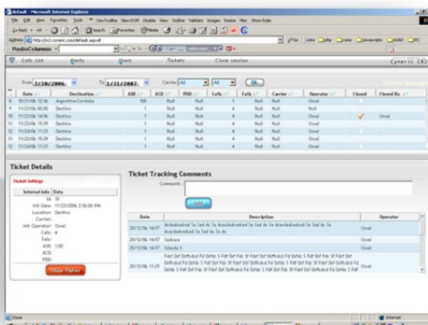
Tickets details
