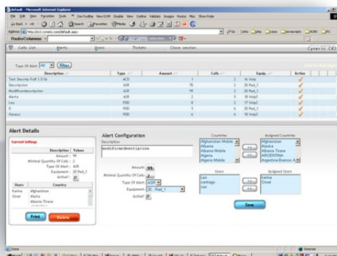
Alert details
