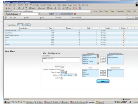
New alert
