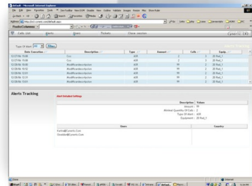
Alerts tracking
